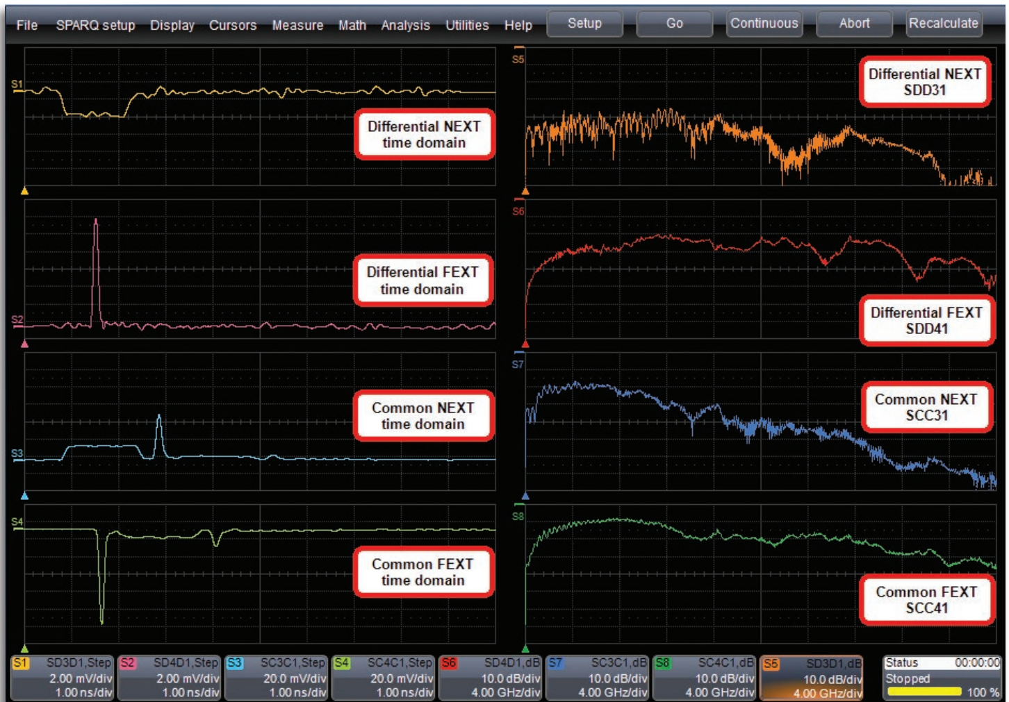
8 and 12-port SPARQs measure both near-end and far-end crosstalk (NEXT and FEXT). In this screenshot, both time-domain and S-parameters are displayed for the differential and common signal crosstalk.
