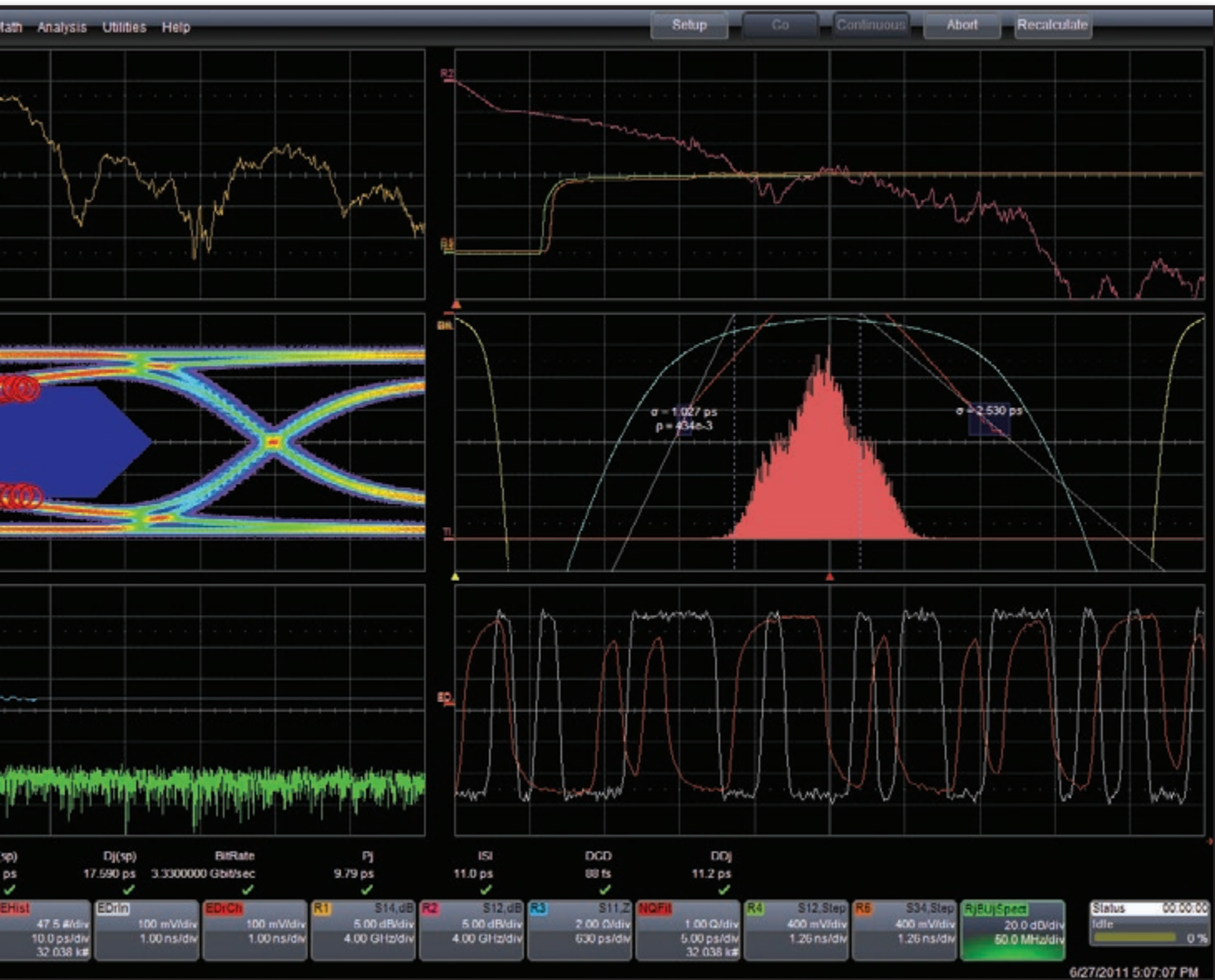
Signal Integrity Studio enhances the modeling and simulation capabilities of the Teledyne LeCroy SPARQ application, adding eye and jitter measurements.
