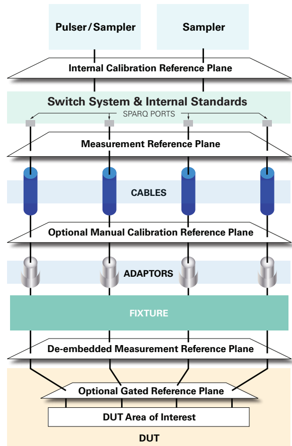
The SPARQ maintains three reference planes – calibration, measurement, and de-embedded DUT. It keeps items that drift with time and temperature behind the calibration reference plane.
