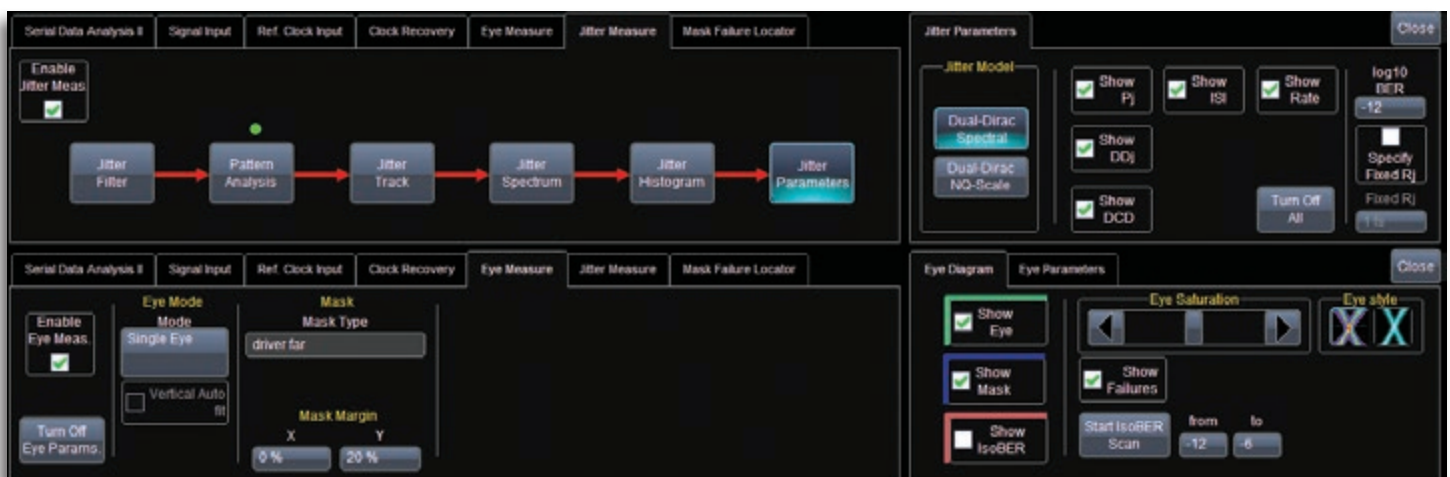
A rich set of jitter and eye diagram analysis tools yield deep insight signal integrity issues of the device under test.
