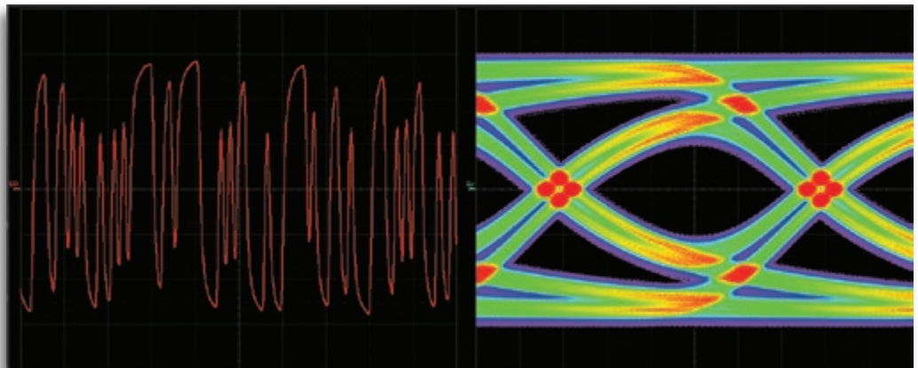
With SI Studio, users can see what the waveform would look like after channel impairments, and view the corresponding eye
