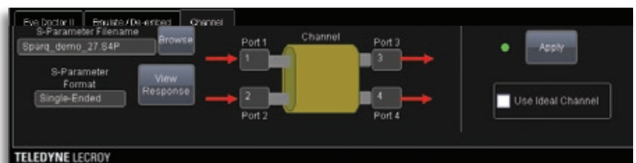
Channels are de-embedded or emulated using either modeled or measured S-parameters.
