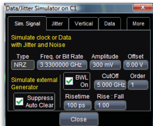
SI Studio utilizes a versatile built-in simulator as a signal source
